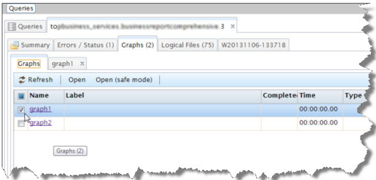
Figure 11. Graphs list
